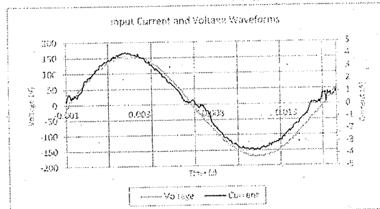
Input AC Current Waveform (I THD = 9.54%, 50% Load)
