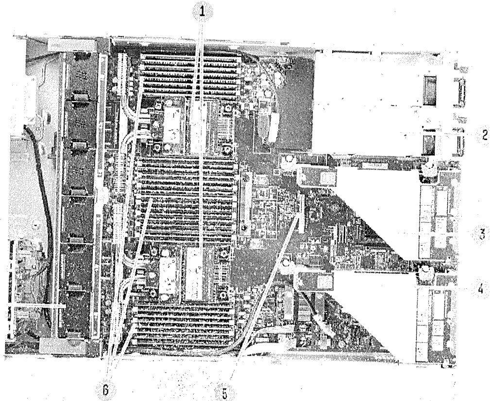
Internal View 8SFF chassis
