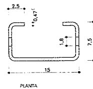
POSTE C-150 P/ DEFENSAS
